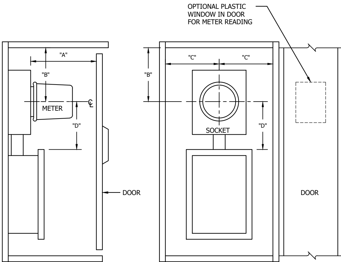
SIDE VIEW
